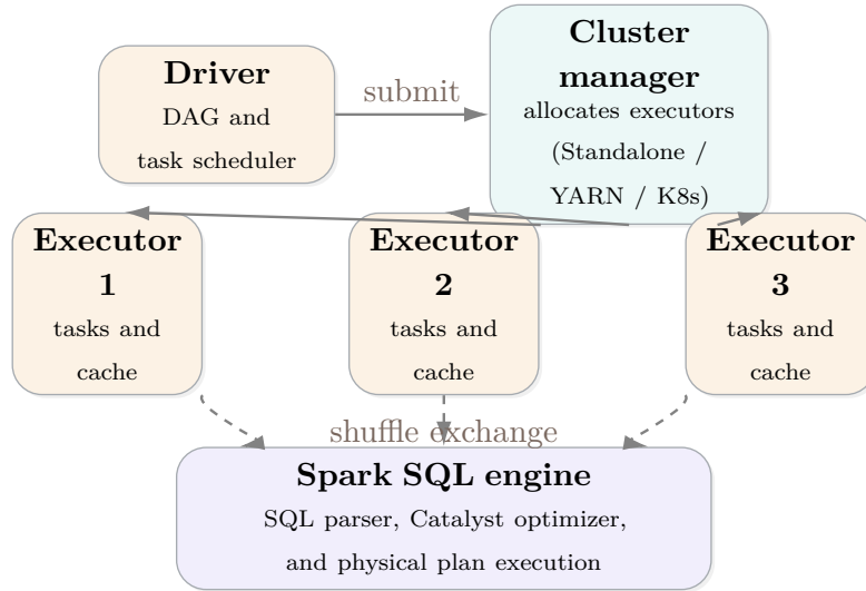
Figure II.2: Conceptual view of distributed execution in a Spark-style compute model.
